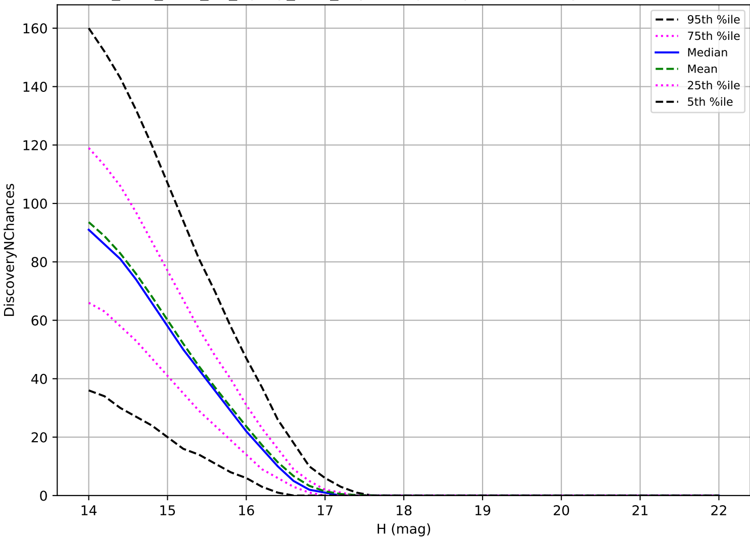
too_elab_r256_d2_ugrizy_v3.4_10yrs: Trojan 3 pairs in 15 nights detection loss
