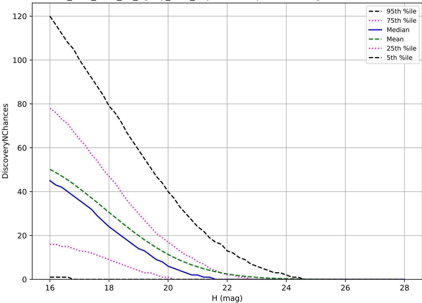
too_elab_r256_d2_ugrizy_v3.4_10yrs: PHA 3 pairs in 15 nights detection loss
