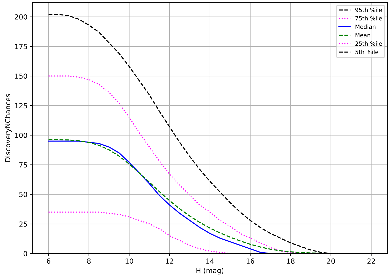
too_elab_r256_d2_ugrizy_v3.4_10yrs: OCC_r5 3 pairs in 15 nights detection loss
