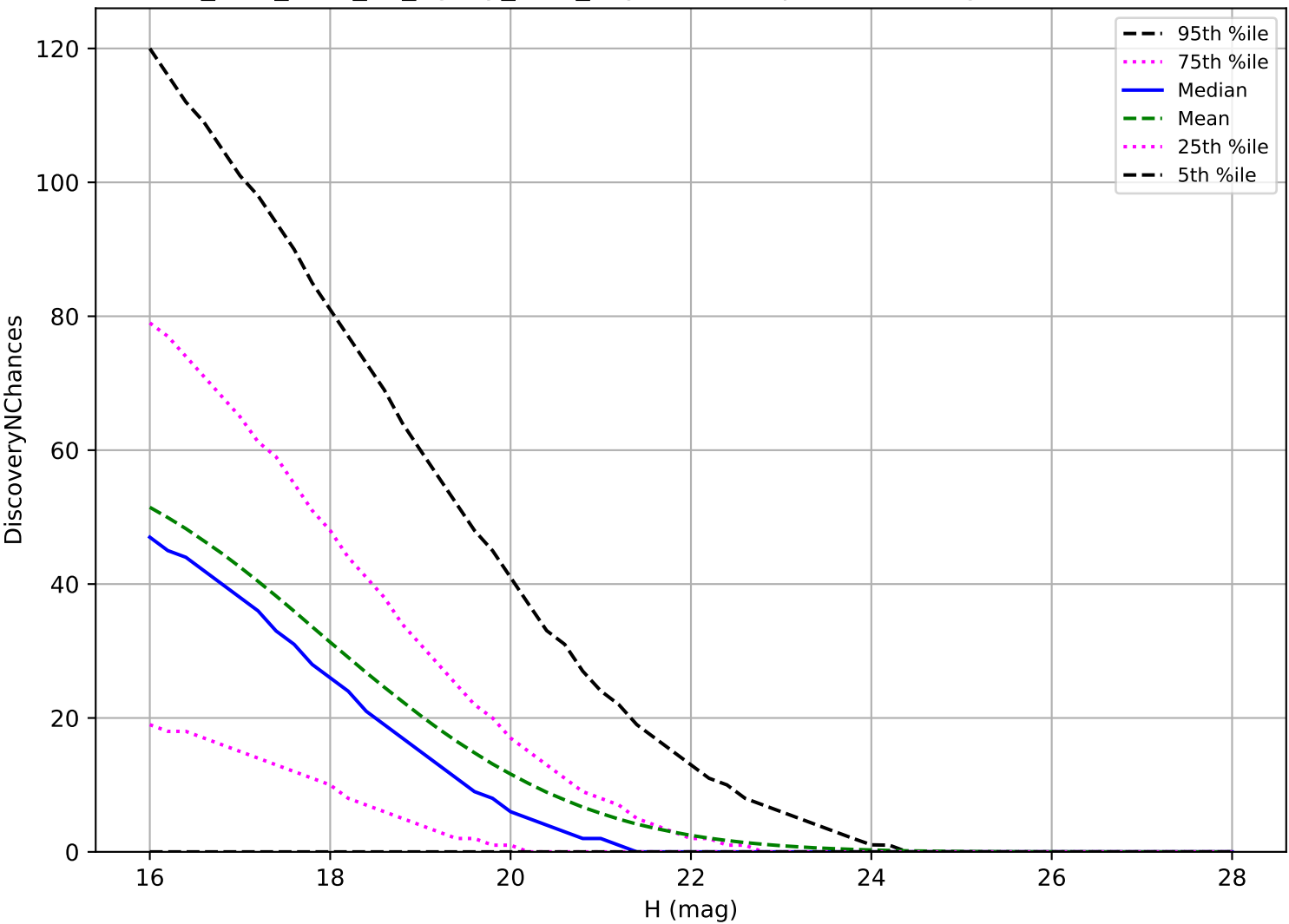
too_elab_r256_d2_ugrizy_v3.4_10yrs: NEO 3 pairs in 15 nights detection loss
