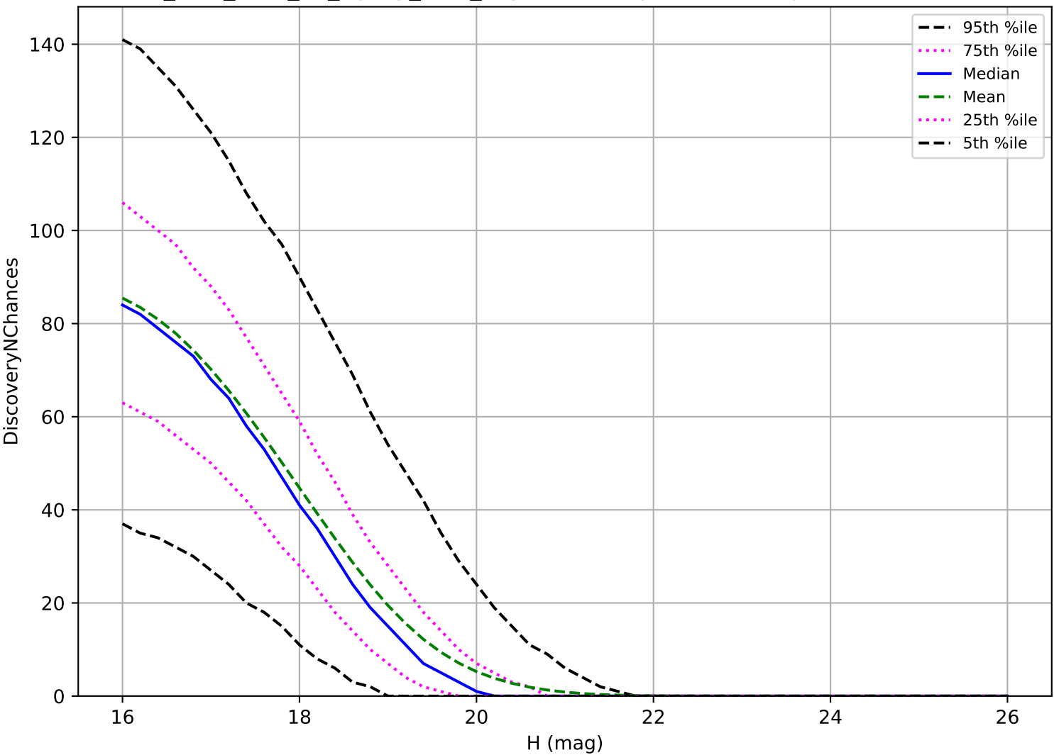
too_elab_r256_d2_ugrizy_v3.4_10yrs: MBA 3 pairs in 15 nights detection loss
