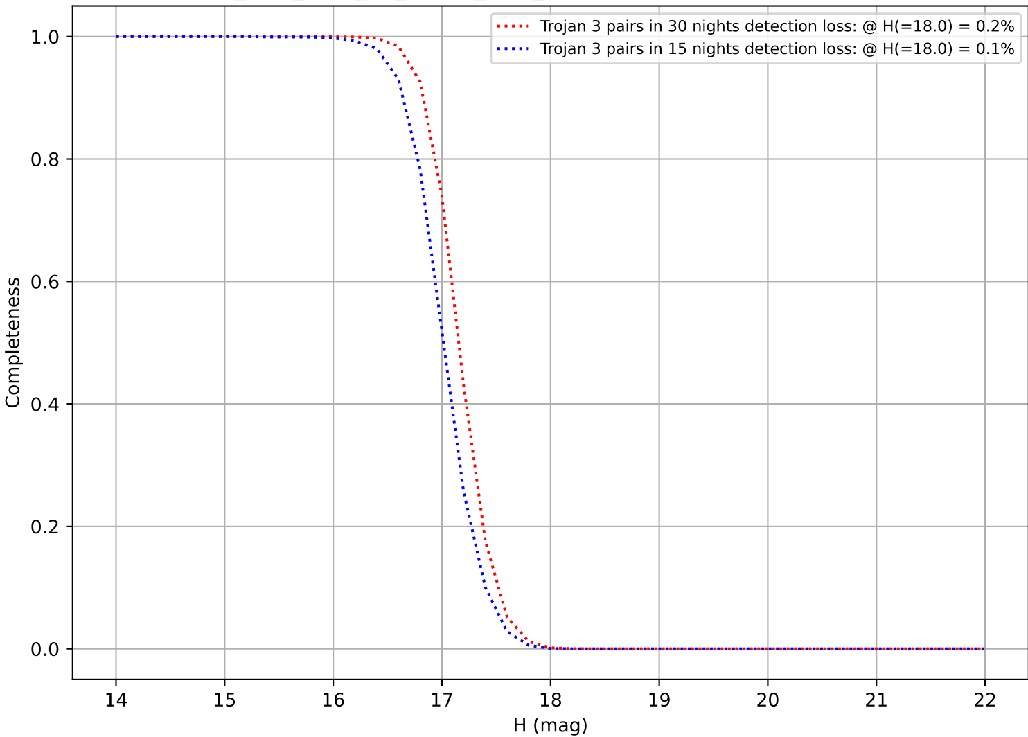
too_elab_r256_d2_ugrizy_v3.4_10yrs: DifferentialCompleteness
