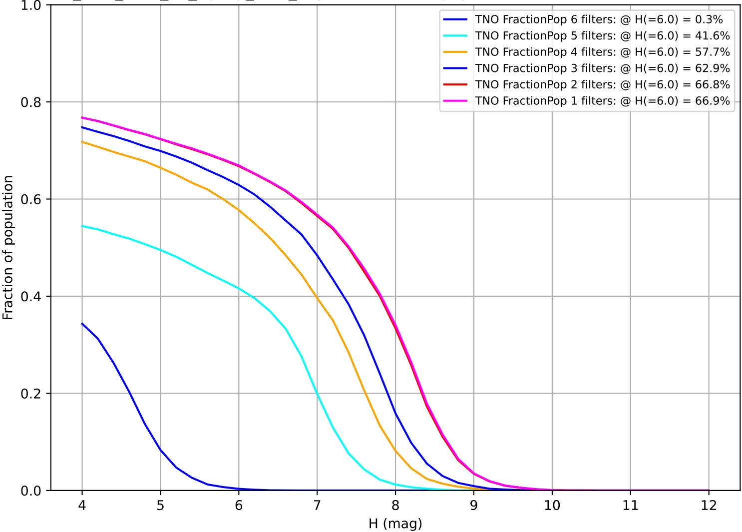
too_elab_r256_d2_ugrizy_v3.4_10yrs: Fraction of population with colors in X filters TNO
