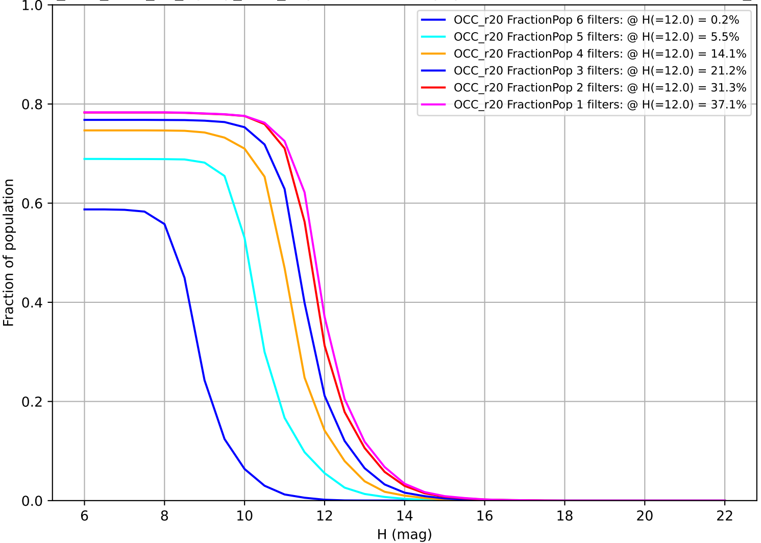
too_elab_r256_d2_ugrizy_v3.4_10yrs: Fraction of population with colors in X filters OCC_r20
