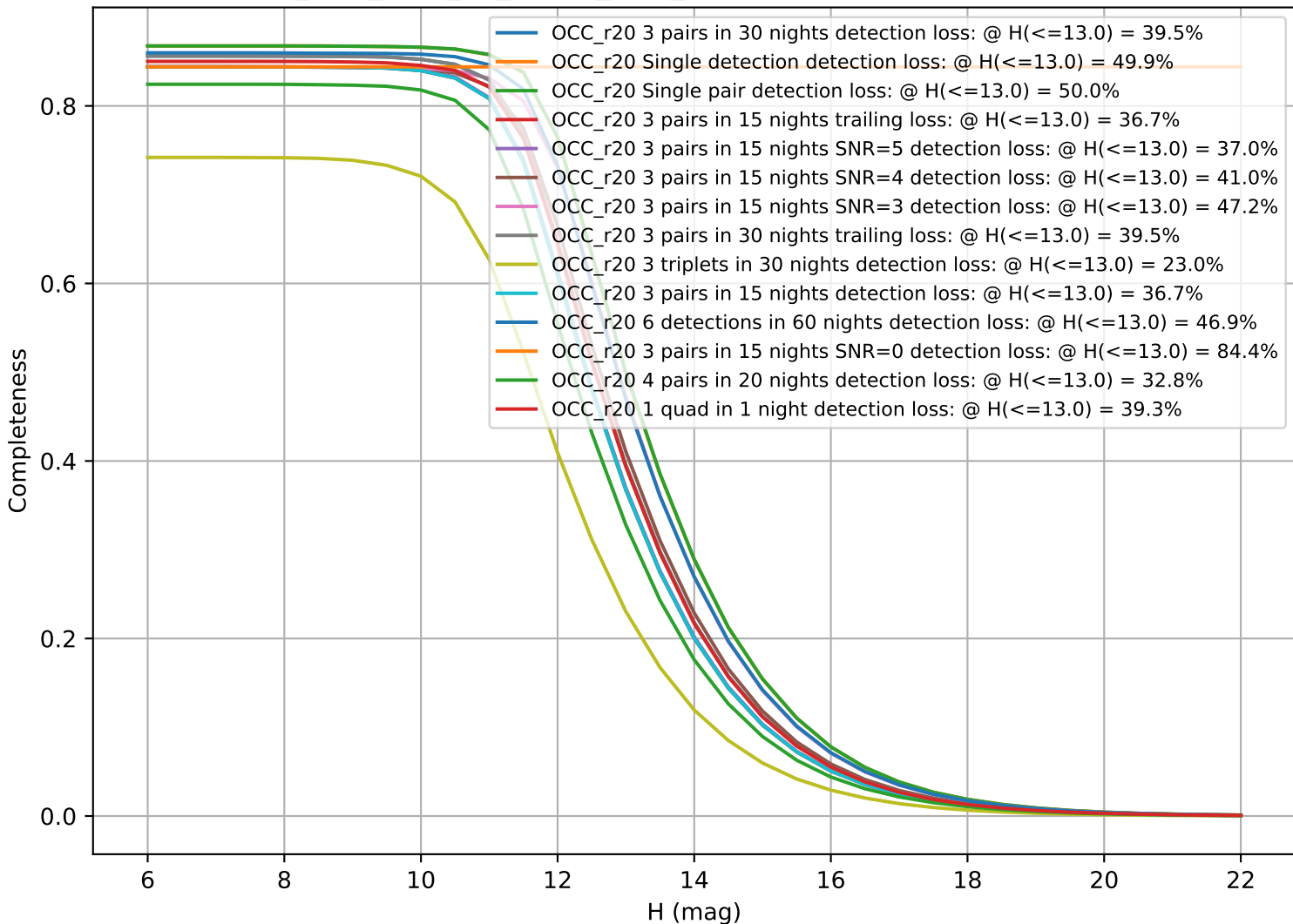
too_elab_r256_d2_ugrizy_v3.4_10yrs: CumulativeCompleteness
