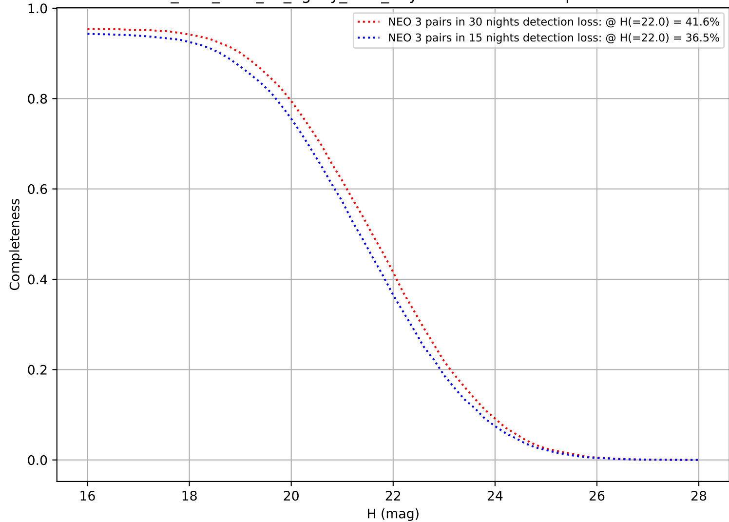
too_elab_r256_d2_ugrizy_v3.4_10yrs: DifferentialCompleteness
