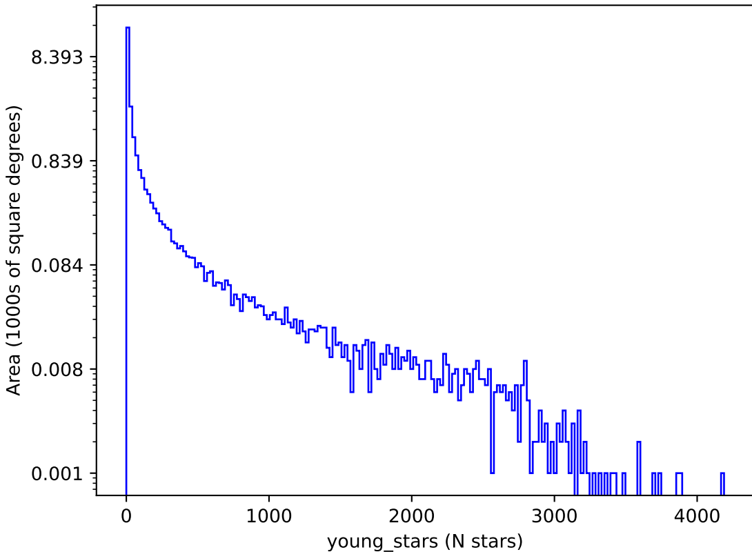
too_elab_r256_d2_ugrizy_v3.4_10yrs : young_stars
