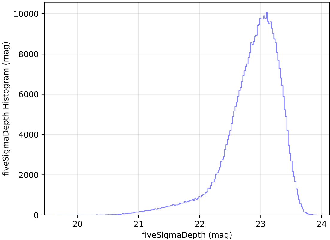
too_elab_r256_d2_ugrizy_v3.4_10yrs z: fiveSigmaDepth Histogram
