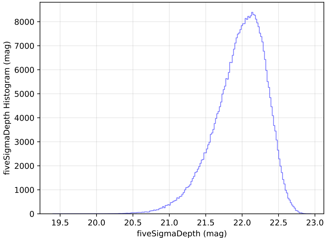
too_elab_r256_d2_ugrizy_v3.4_10yrs y: fiveSigmaDepth Histogram
