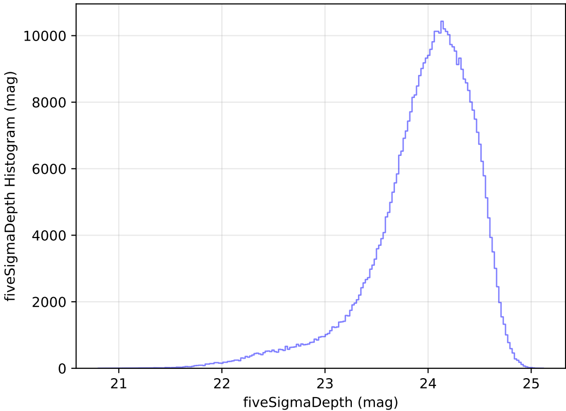
too_elab_r256_d2_ugrizy_v3.4_10yrs r: fiveSigmaDepth Histogram
