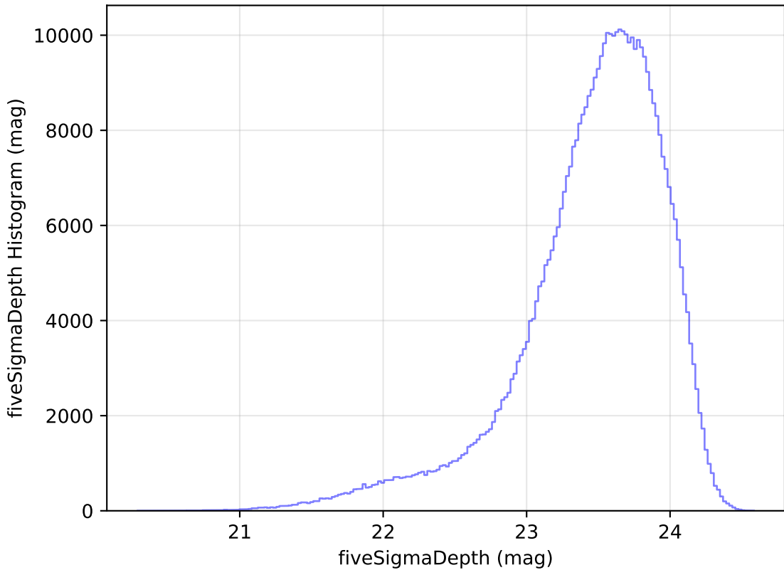
too_elab_r256_d2_ugrizy_v3.4_10yrs i: fiveSigmaDepth Histogram
