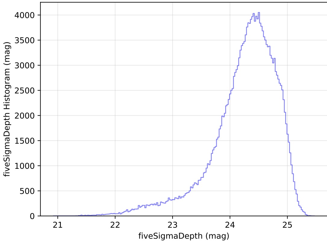
too_elab_r256_d2_ugrizy_v3.4_10yrs g: fiveSigmaDepth Histogram
