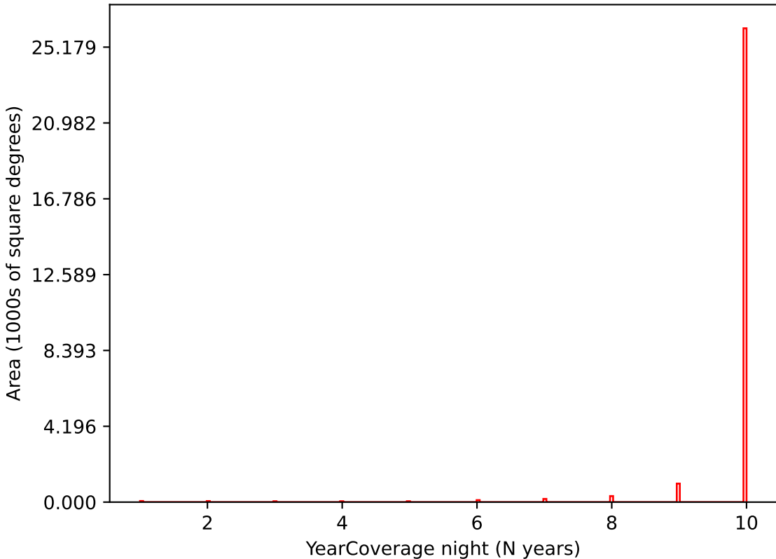
too_elab_r256_d2_ugrizy_v3.4_10yrs i band: YearCoverage night
