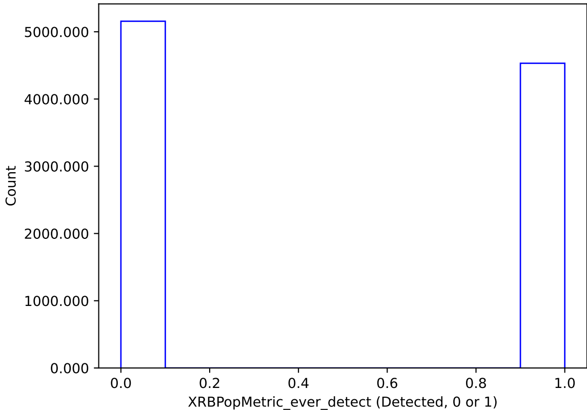
too_elab_r256_d2_ugrizy_v3.4_10yrs : XRBPoMetric_ever_detect
