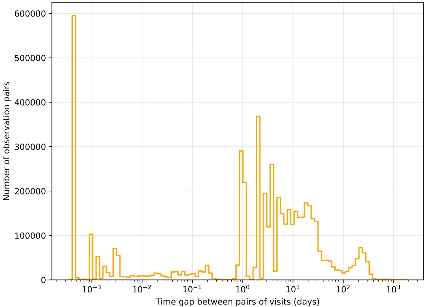
too_elab_r256_d2_ugrizy_v3.4_10yrs r band: Tgaps observationStartMJD
