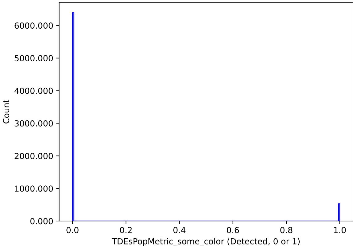
too_elab_r256_d2_ugrizy_v3.4_10yrs : TDEsPopMetric_some_color
