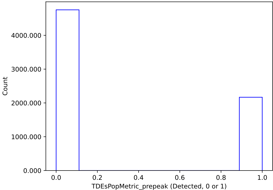
too_elab_r256_d2_ugrizy_v3.4_10yrs : TDEsPopMetric_prepeak
