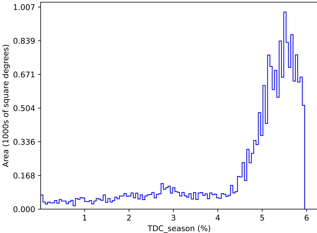
too_elab_r256_d2_ugrizy_v3.4_10yrs : TDC_season
