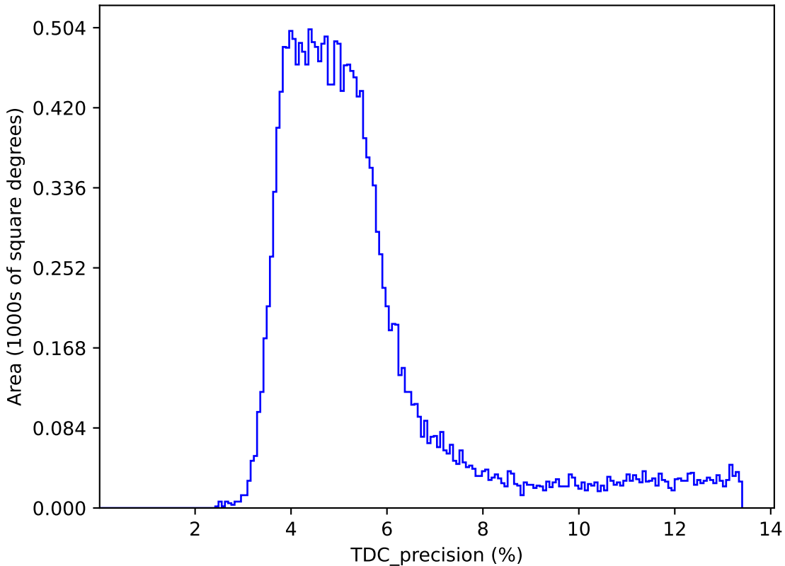
too_elab_r256_d2_ugrizy_v3.4_10yrs : TDC_precision
