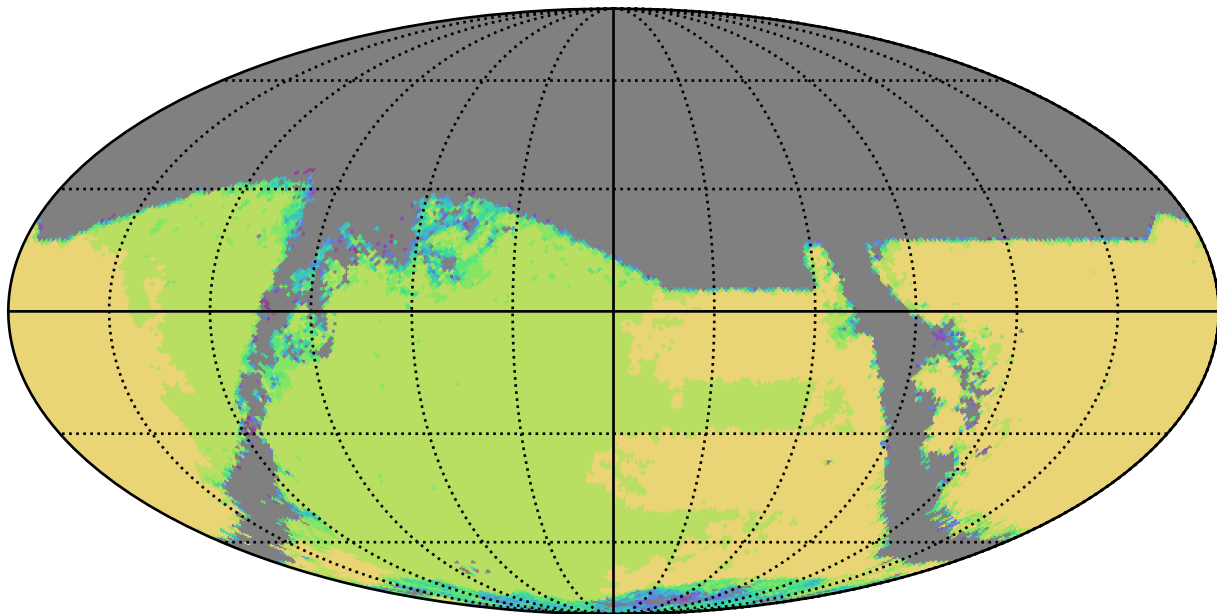
too_elab_r256_d2_ugrizy_v3.4_10yrs : TDC_campaign
