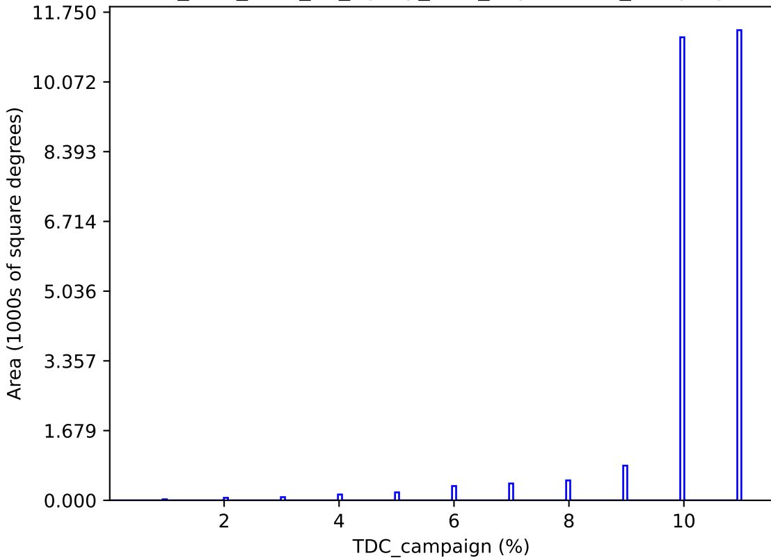
too_elab_r256_d2_ugrizy_v3.4_10yrs : TDC_campaign
