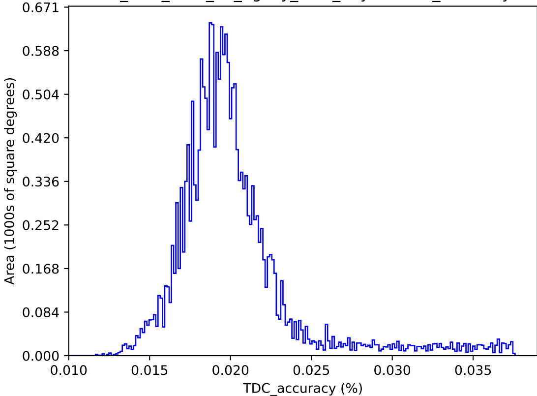
too_elab_r256_d2_ugrizy_v3.4_10yrs : TDC_accuracy
