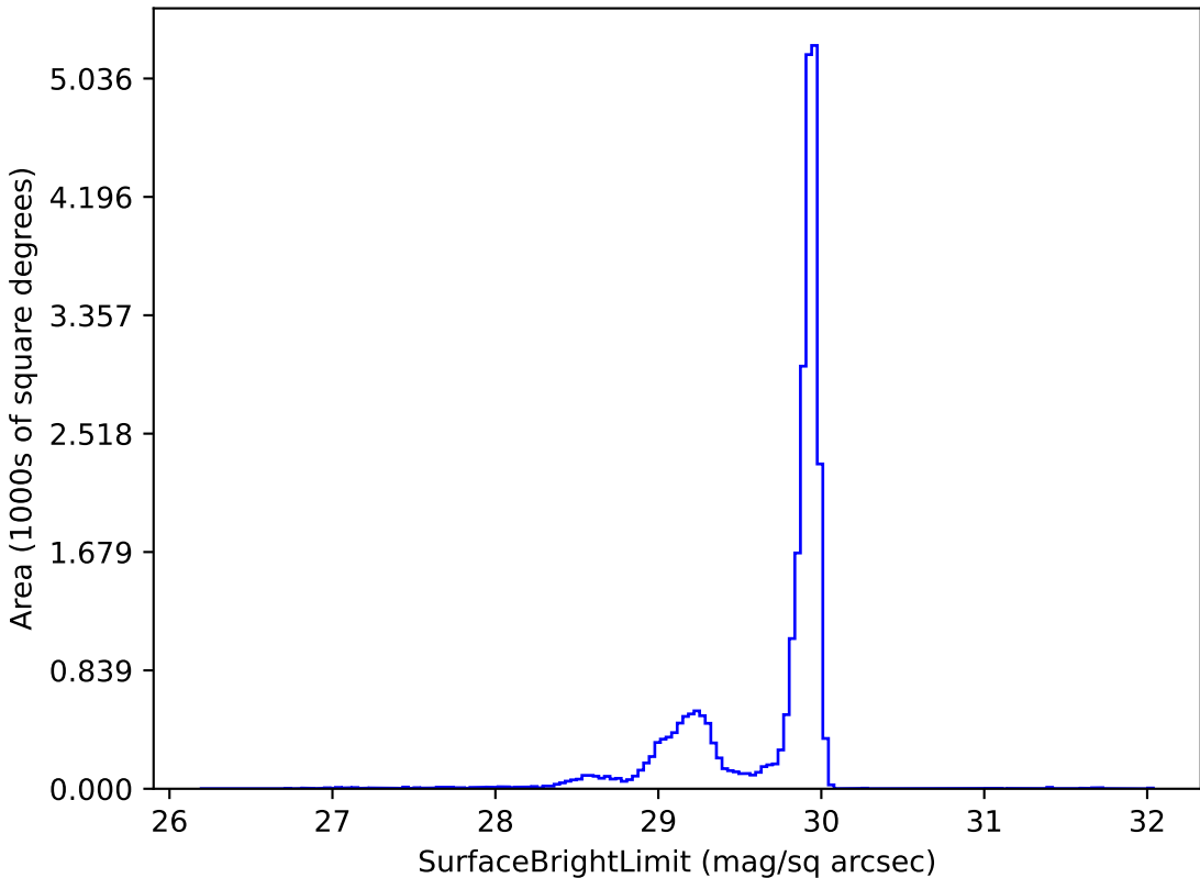
too_elab_r256_d2_ugrizy_v3.4_10yrs i: SurfaceBrightLimit
