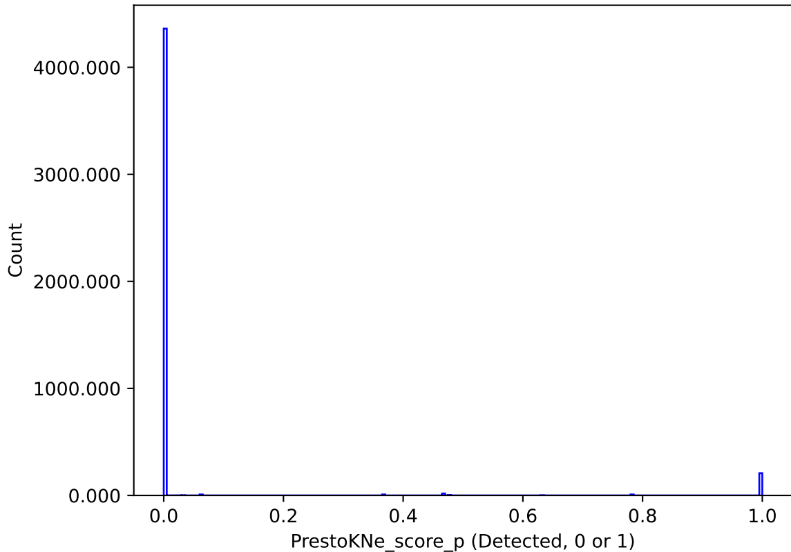
too_elab_r256_d2_ugrizy_v3.4_10yrs : PrestoKNe_score_p
