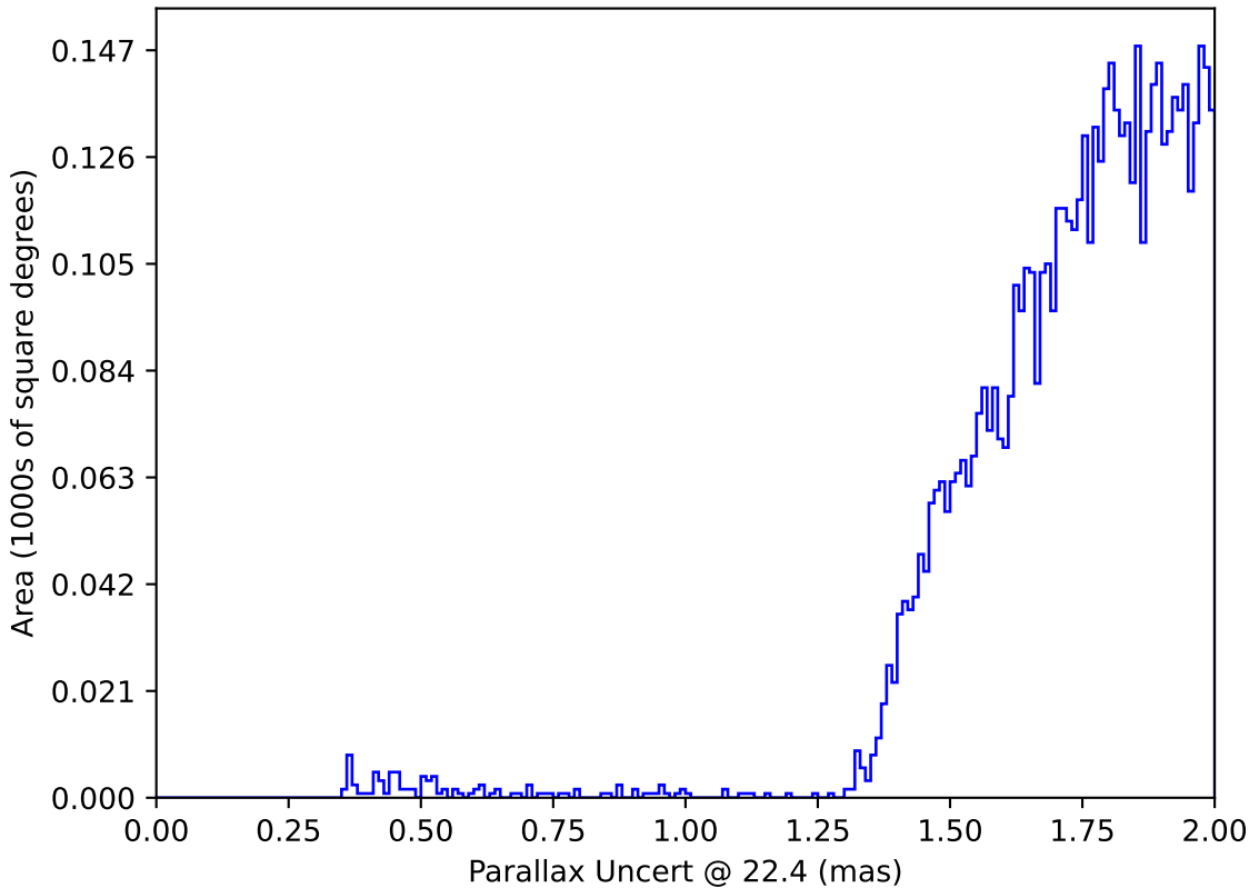
too_elab_r256_d2_ugrizy_v3.4_10yrs : Parallax Uncert @ 22.4
