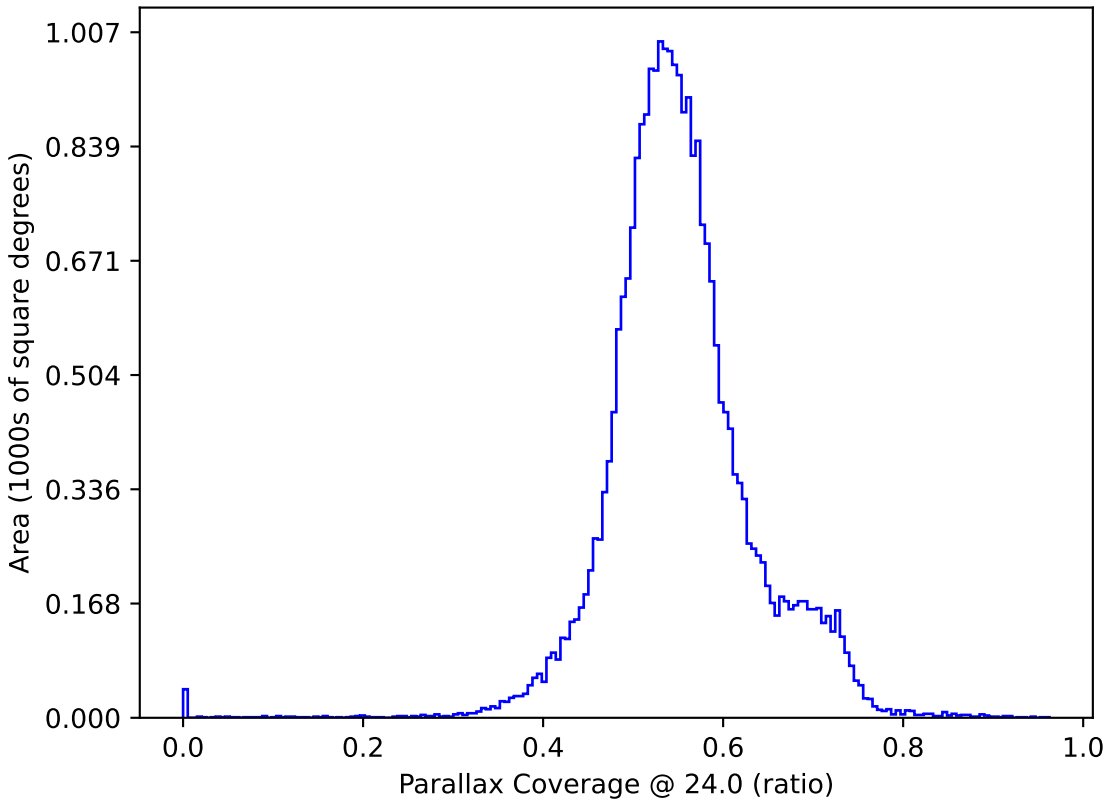
too_elab_r256_d2_ugrizy_v3.4_10yrs : Parallax Coverage @ 24.0
