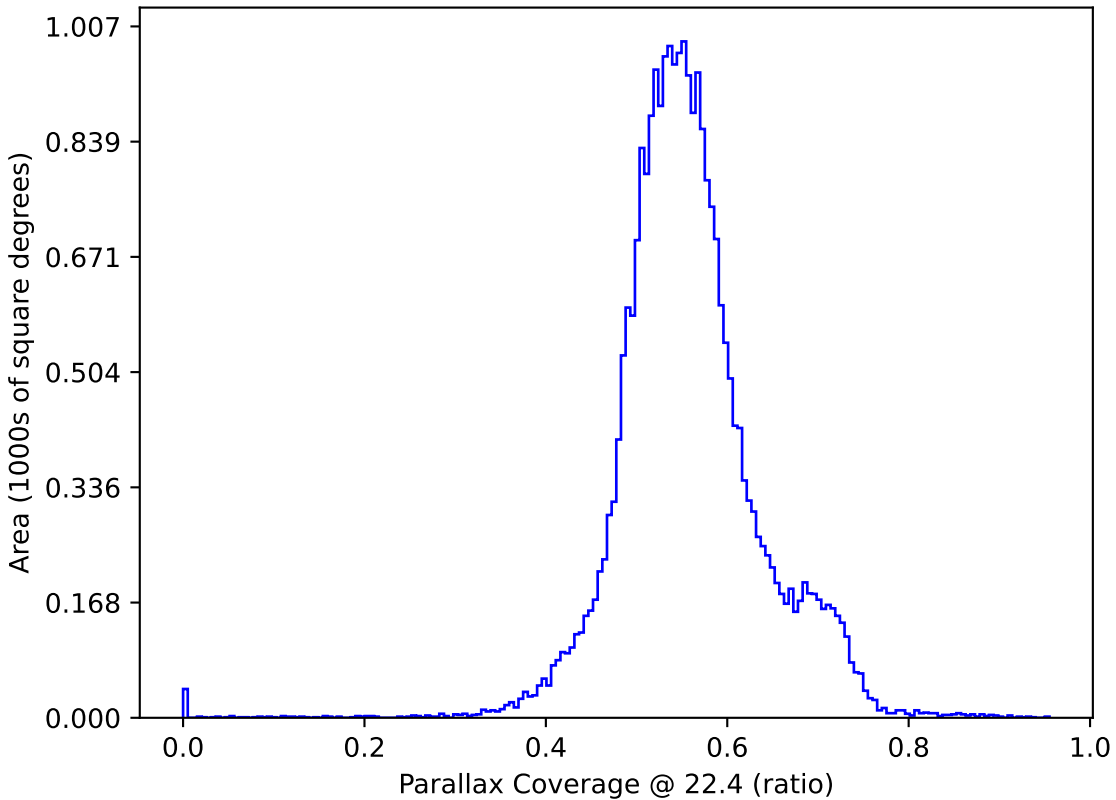
too_elab_r256_d2_ugrizy_v3.4_10yrs : Parallax Coverage @ 22.4
