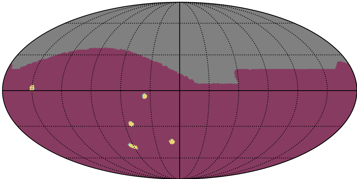
too_elab_r256_d2_ugrizy_v3.4_10yrs : NumberOfQuickRevisits
