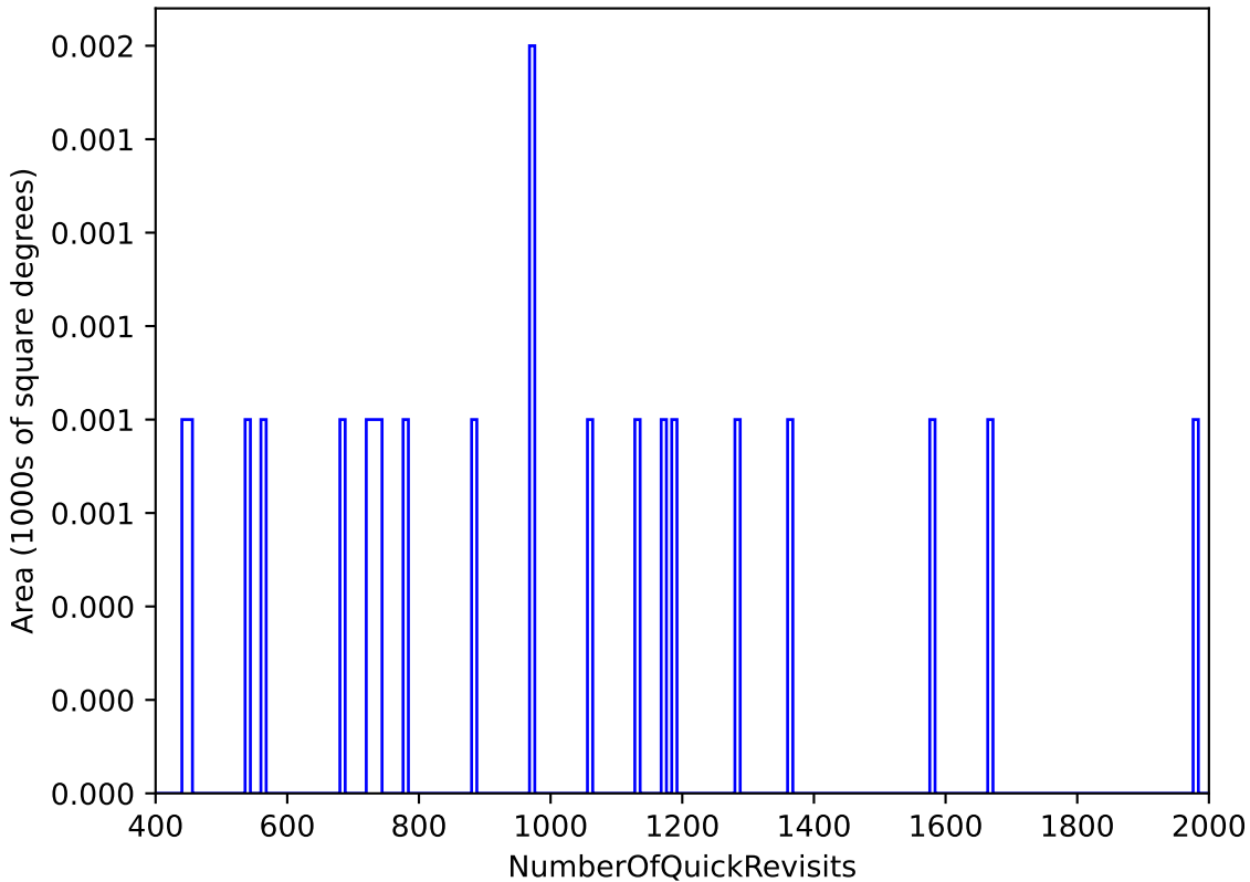
too_elab_r256_d2_ugrizy_v3.4_10yrs : NumberOfQuickRevisits
