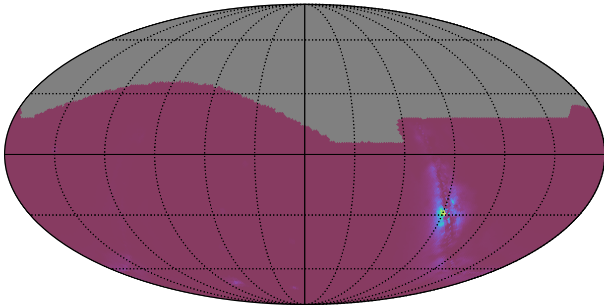
too_elab_r256_d2_ugrizy_v3.4_10yrs : NlcPoints
