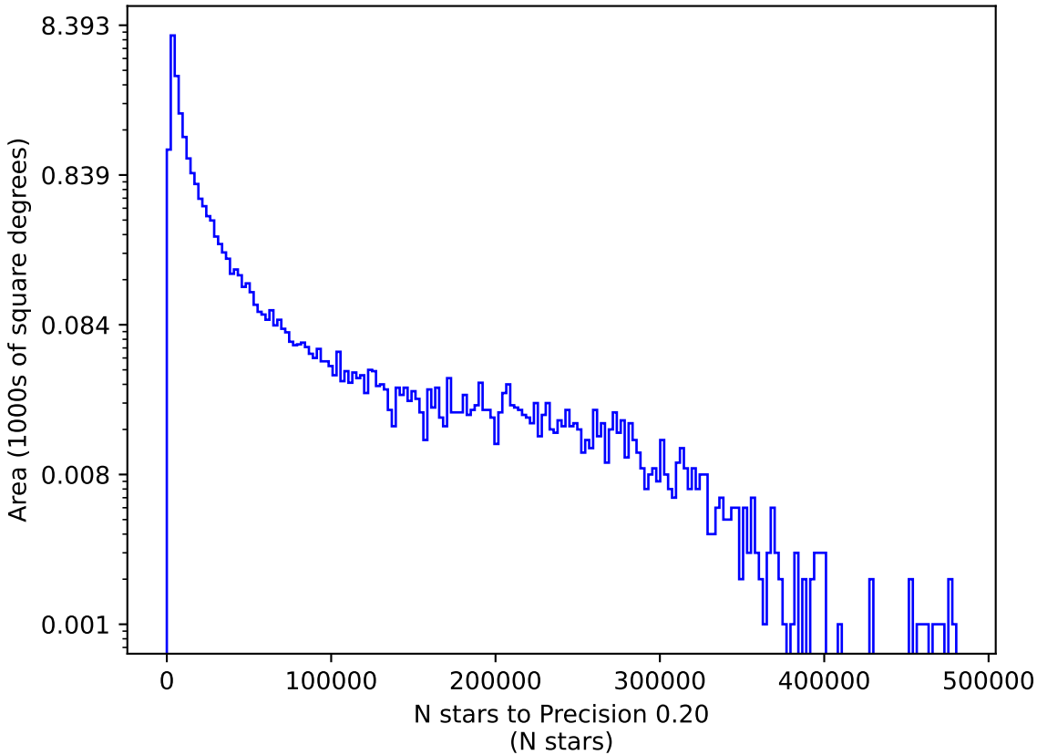
too_elab_r256_d2_ugrizy_v3.4_10yrs u: N stars to Precision 0.20
