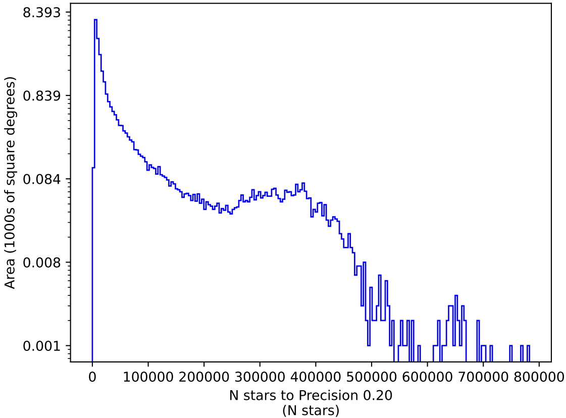
too_elab_r256_d2_ugrizy_v3.4_10yrs g: N stars to Precision 0.20
