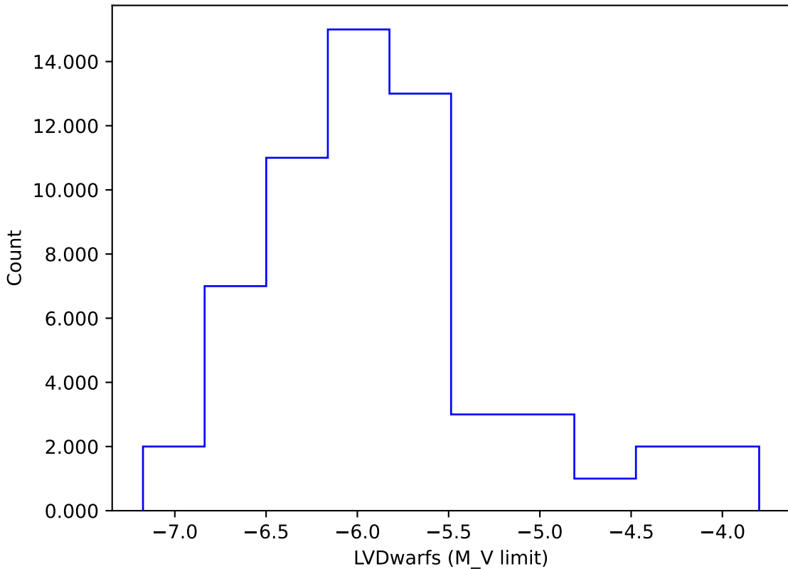
too_elab_r256_d2_ugrizy_v3.4_10yrs gi: LVDwarfs
