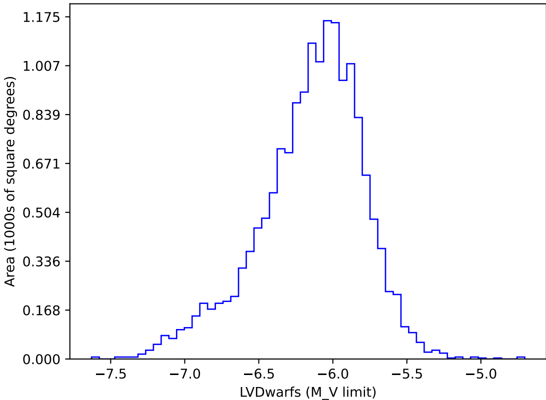
too_elab_r256_d2_ugrizy_v3.4_10yrs gi: LVDwarfs
