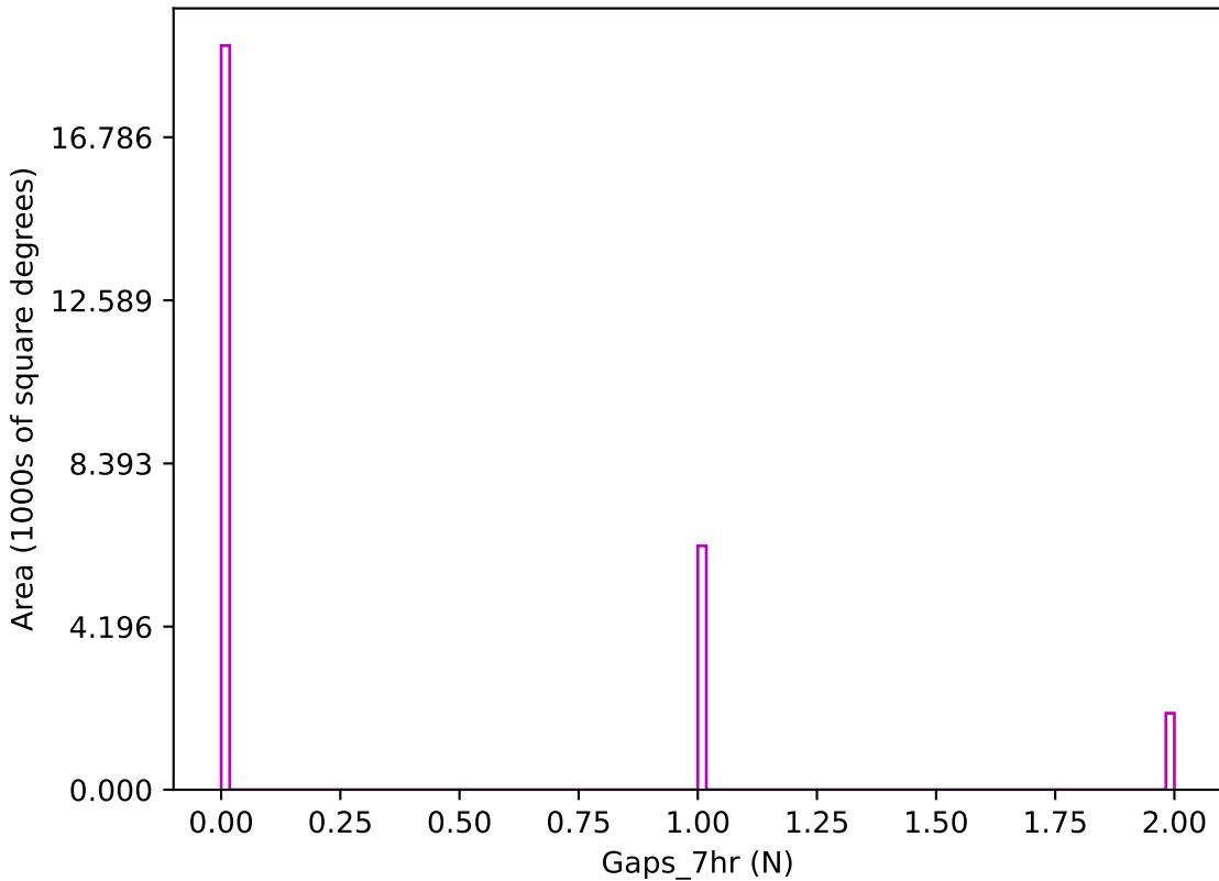
too_elab_r256_d2_ugrizy_v3.4_10yrs z band: Gaps_7hr
