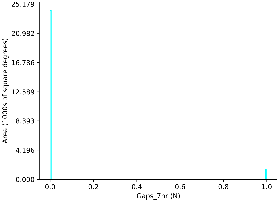
too_elab_r256_d2_ugrizy_v3.4_10yrs u band: Gaps_7hr
