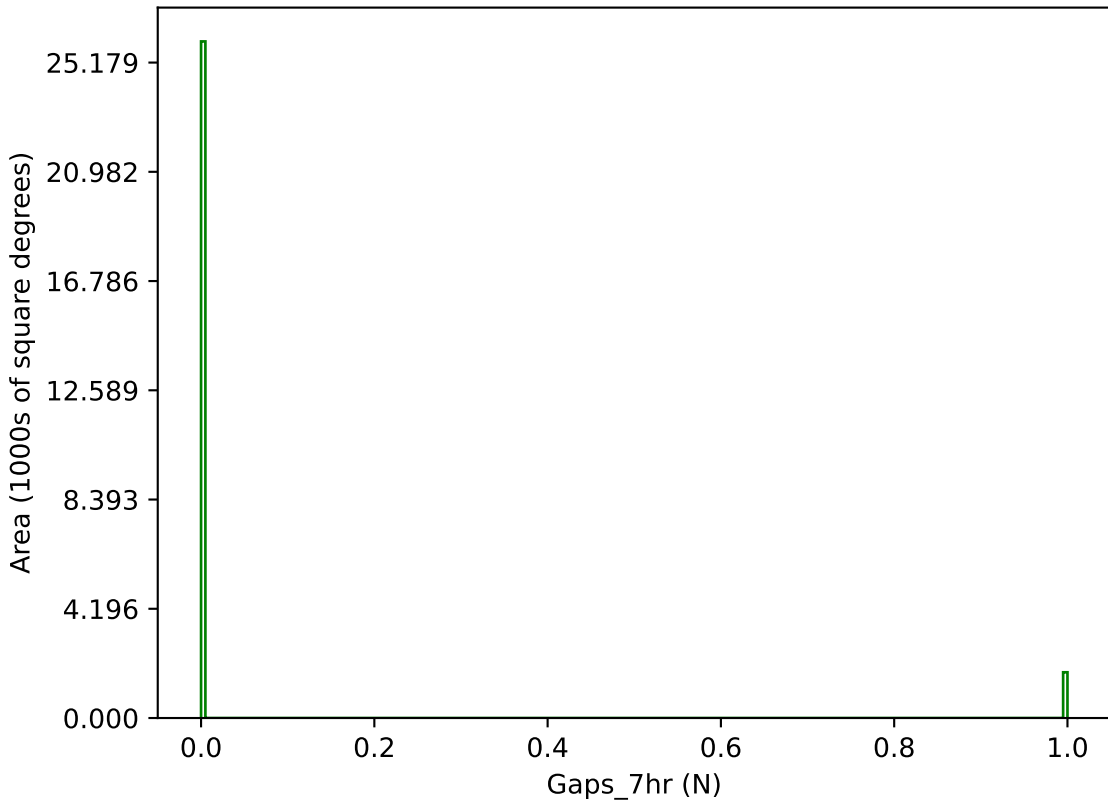
too_elab_r256_d2_ugrizy_v3.4_10yrs g band: Gaps_7hr
