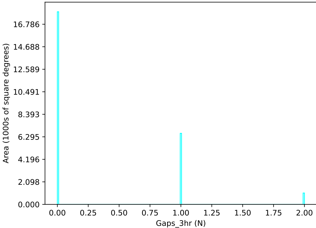
too_elab_r256_d2_ugrizy_v3.4_10yrs u band: Gaps_3hr
