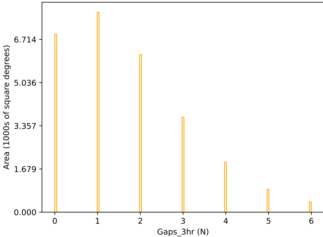
too_elab_r256_d2_ugrizy_v3.4_10yrs r band: Gaps_3hr
