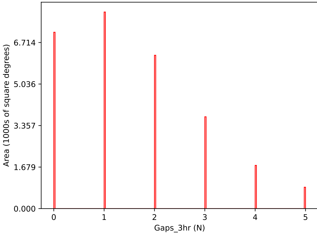
too_elab_r256_d2_ugrizy_v3.4_10yrs i band: Gaps_3hr
