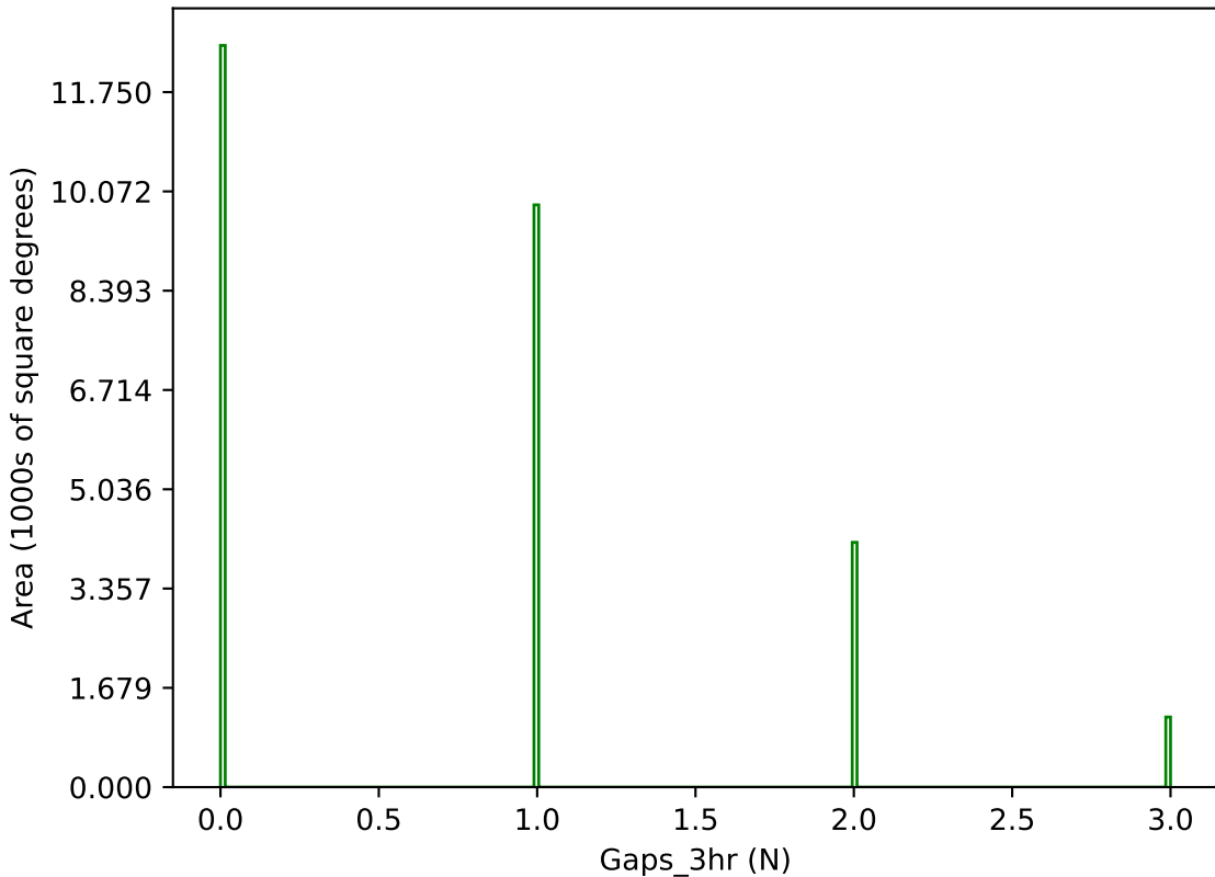
too_elab_r256_d2_ugrizy_v3.4_10yrs g band: Gaps_3hr
