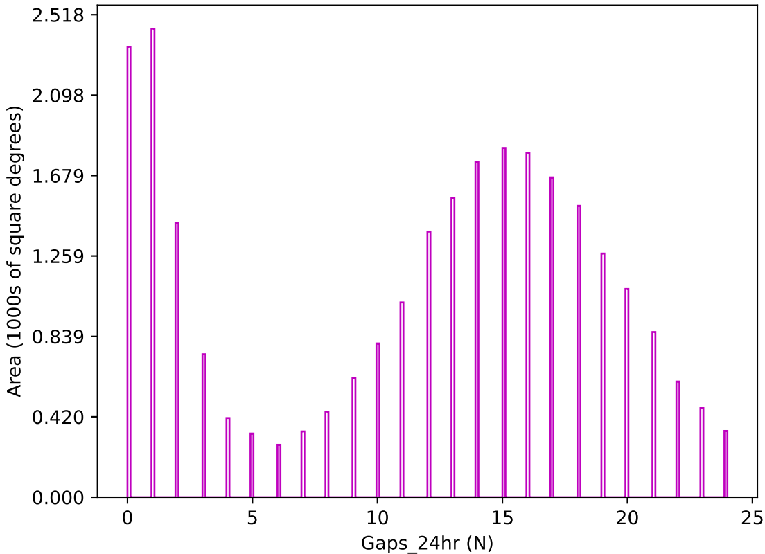
too_elab_r256_d2_ugrizy_v3.4_10yrs z band: Gaps_24hr
