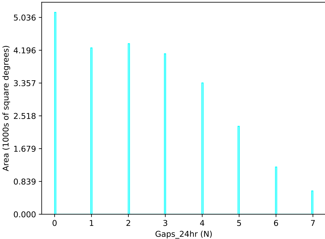
too_elab_r256_d2_ugrizy_v3.4_10yrs u band: Gaps_24hr
