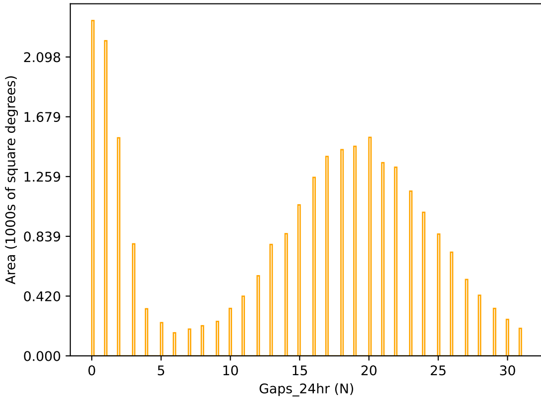
too_elab_r256_d2_ugrizy_v3.4_10yrs r band: Gaps_24hr
