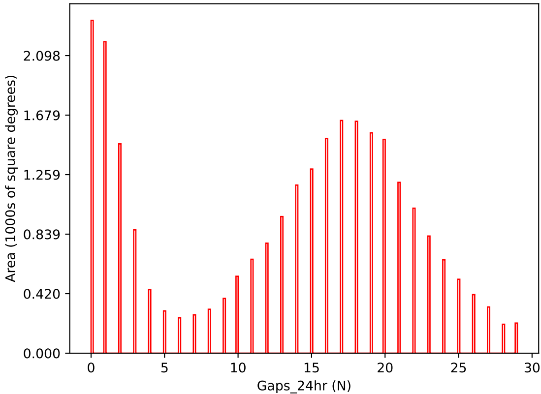
too_elab_r256_d2_ugrizy_v3.4_10yrs i band: Gaps_24hr
