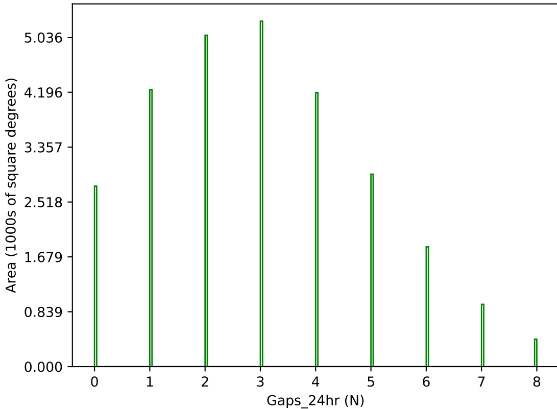
too_elab_r256_d2_ugrizy_v3.4_10yrs g band: Gaps_24hr
